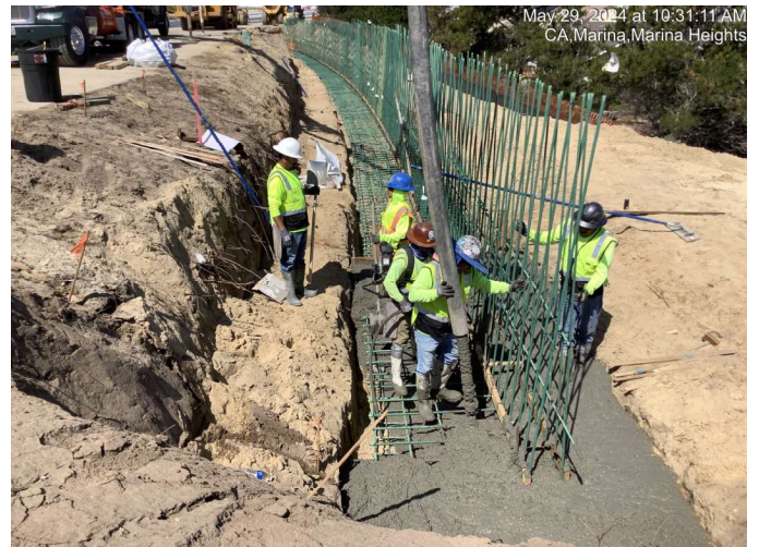
Concrete placed for retaining wall footing near Marina Heights Drive
