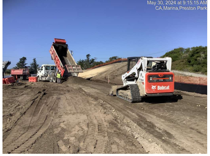
Reusing base rock from old roadway section for subgrade material of new roadway section (near Reservation Road)
